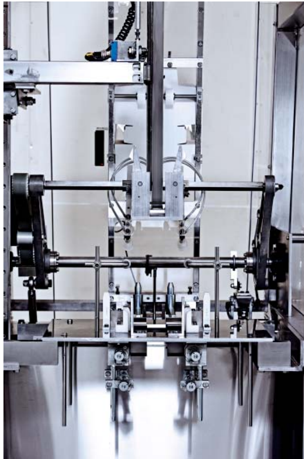
Tool plate and plunger for tool type 301
